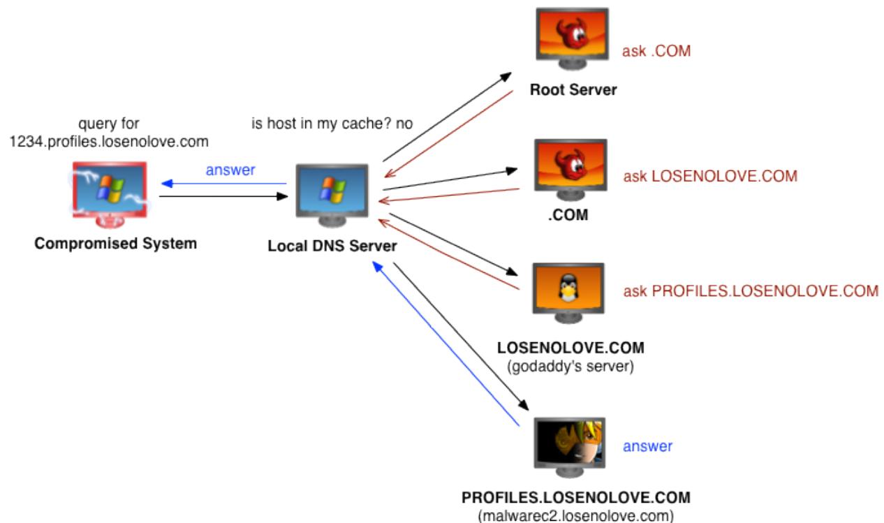
Figure 21. DNS Beacon in Action
