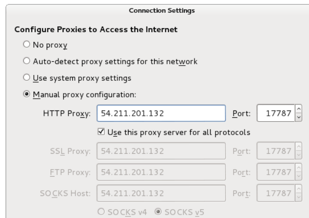
Figure 42. Configure Browser Settings
