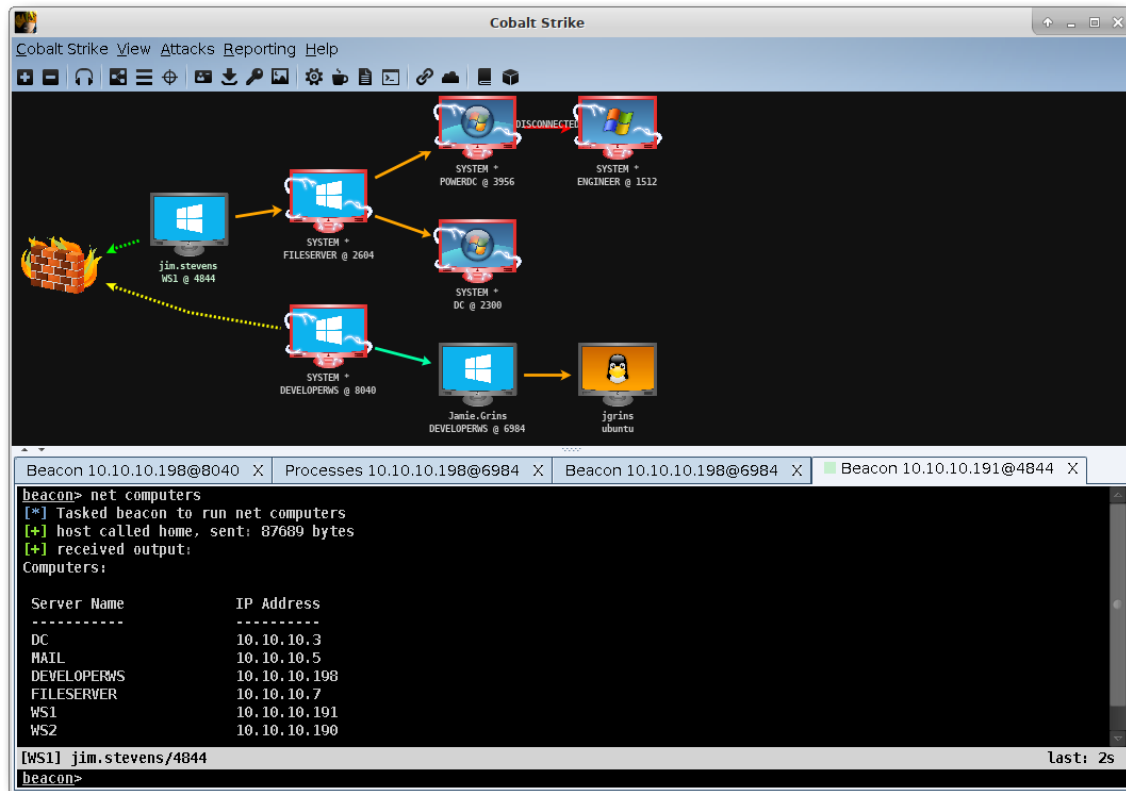
Figure 9. Cobalt Strike User Interface
