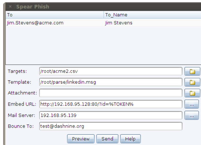
Figure 29. Spear Phishing Tool
